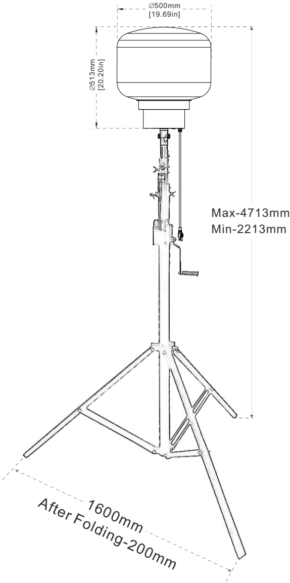
4.3m Tripod
