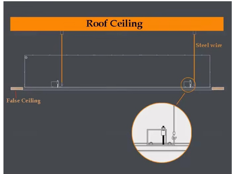
Hanging wire Installation diagram
