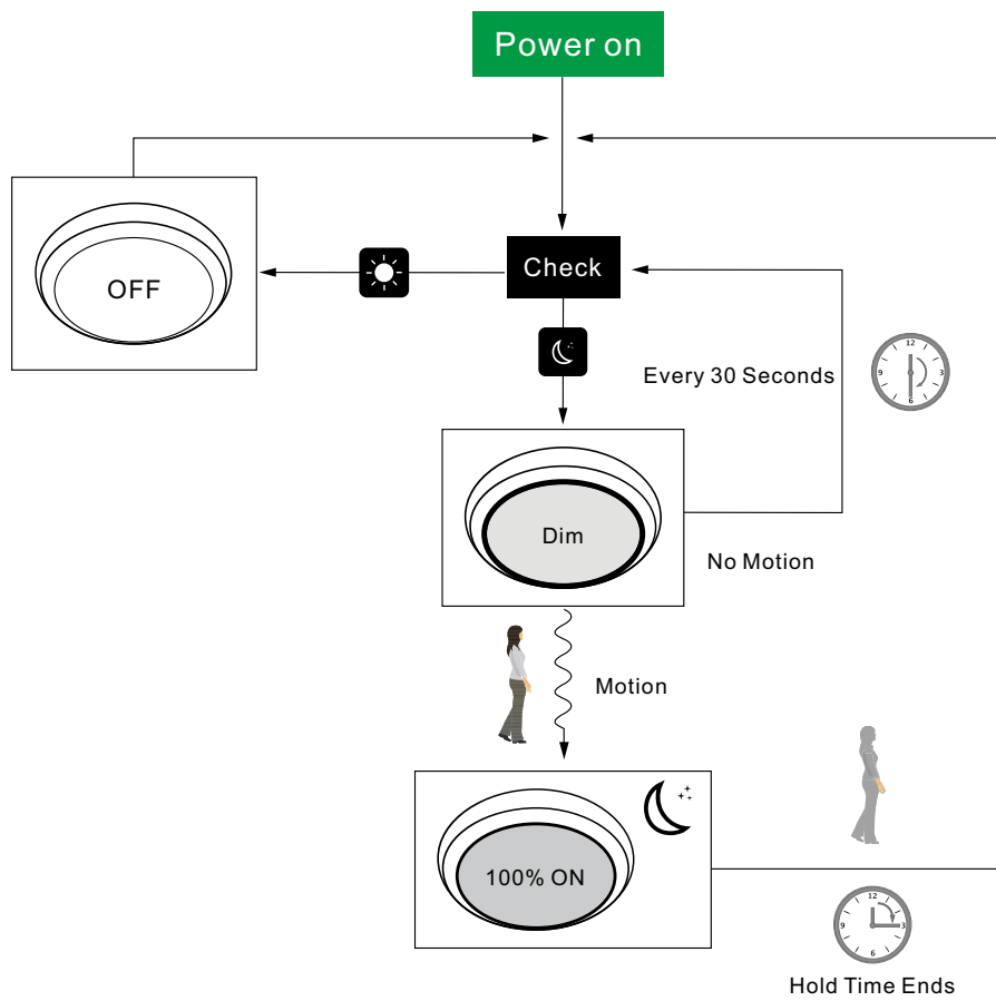
Microwave Sensor
